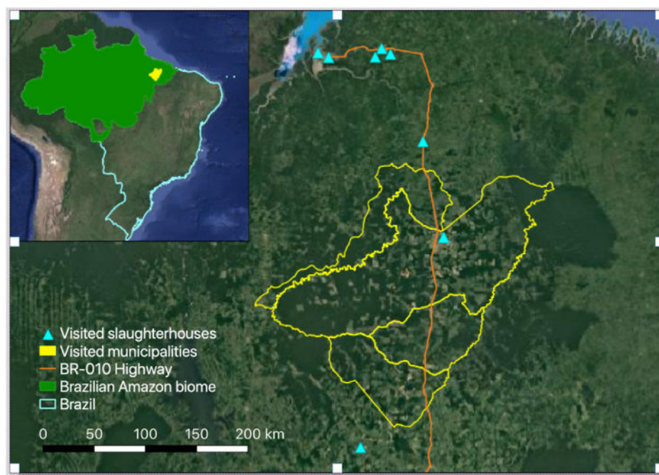
Fig. 2. Study area: From North to South the municipalities are: Ipixuna do Pará, Paragominas, Dom Eliseu and Ulianópolis. Sources: roads: Open Street Map; municipal borders, biome border and national border: Instituto Brasileiro de Geografia e Estatística (IBGE); base layer: Google, 2020.
