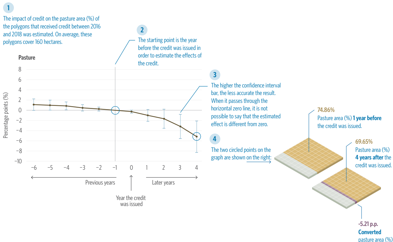
Figure 9. Effects of ABC Recuperação Credit on the Proportion of Total Pasture Area and by Quality Classes over the Polygon Area, 2016–2018
