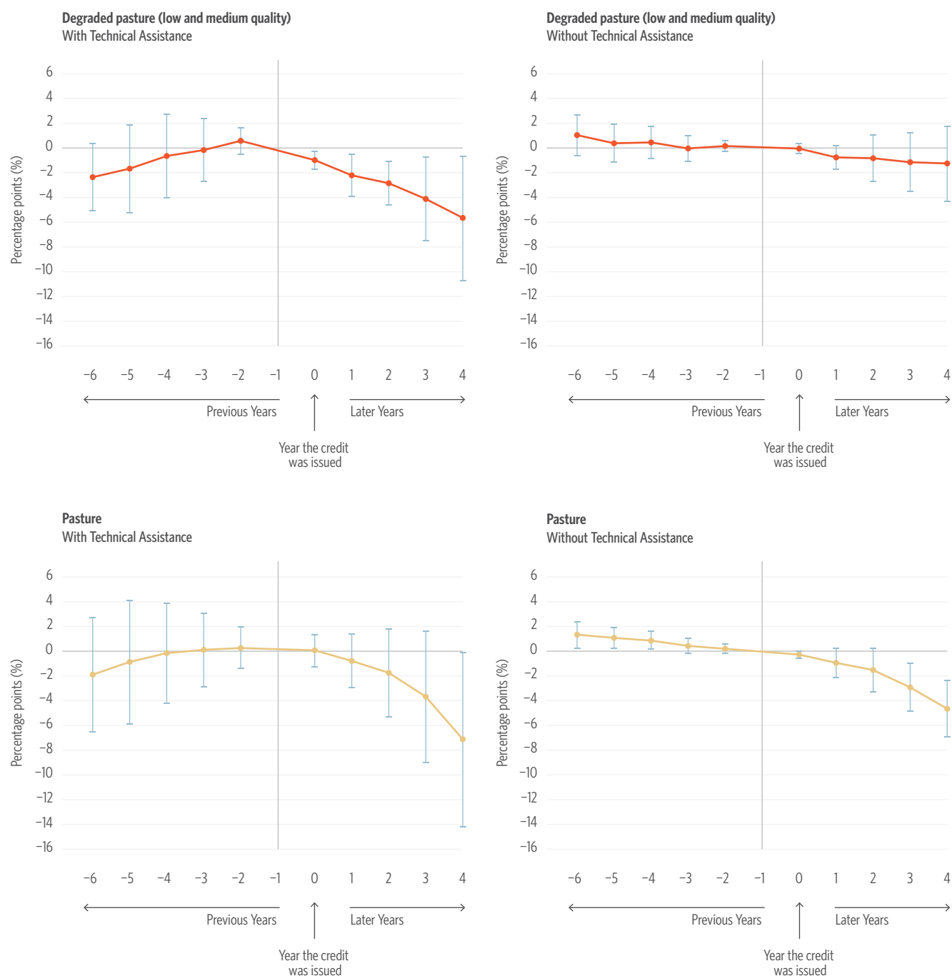
Figure 12. Dynamic Effects of ABC Recuperação Credit on the Proportion of Total Pasture Area and Degraded Pasture (Low or Medium Quality) over the Polygon Area, with and without Technical Assistance, 2016–2018
