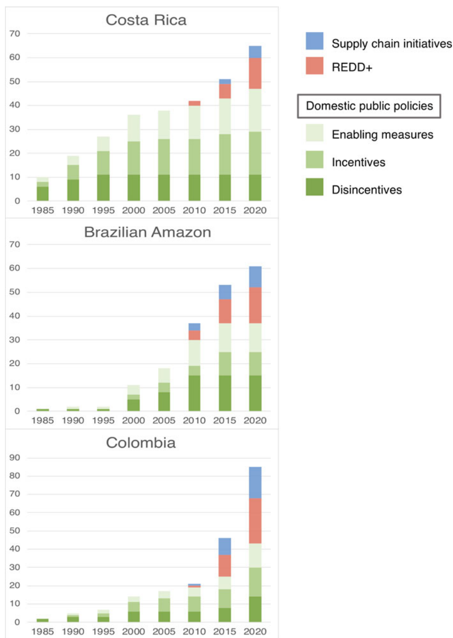
Fig. 2. The evolving policy mix to reduce deforestation in three national case studies from Latin America. Domestic public policies like area-based disincentives and command-and-control measures developed early in the policy sequence, followed by financial incentives to increase compliance. Enabling measures to support (dis)incentives increased at later stages to enhance coordination in the policy mix. REDD+ and supply chain initiatives consist primarily of incentives and enabling measures. Graph values represent cumulative interventions in the policy mix prior to, but not including, the year displayed in each column.
