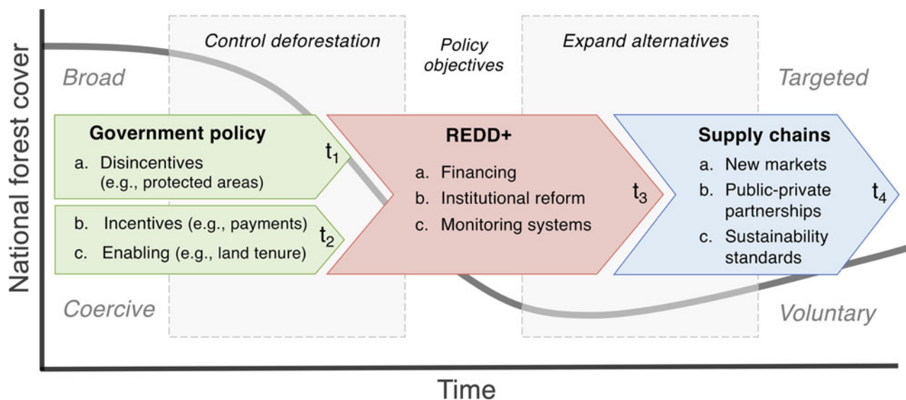
Fig. 3. Stages of policy sequencing along the forest transition curve. Earlier in the forest transition, coercive instruments are designed to control deforestation and disrupt lock-in of existing production models. Instruments become more targeted with the deployment of incentives. Later in the forest transition, voluntary instruments expand alternative models of sustainable production that lead to forest recovery. The policy sequence ( t_n ) represents the addition of (not transition to) new actor domains as interventions are layered into the policy mix.
