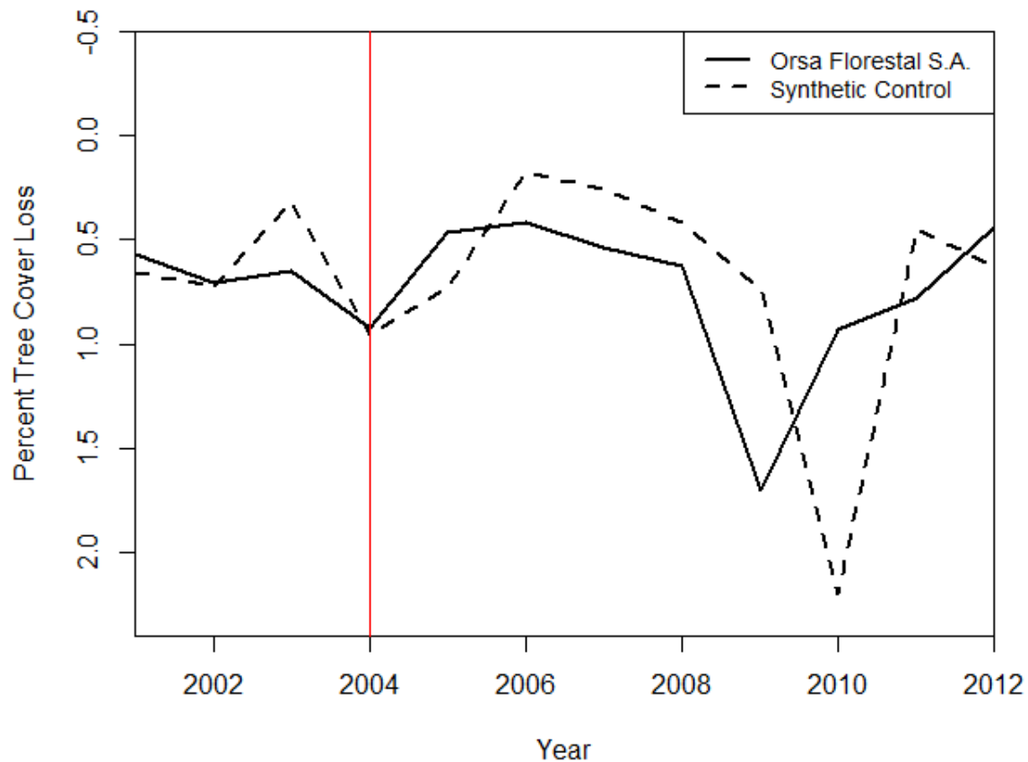
Figure 2. Comparison of tree cover loss in Orsa Florestal S.A. and its synthetic control, 2001–2012. Tree cover loss increases down the y -axis. Red line indicates the year of certification.
