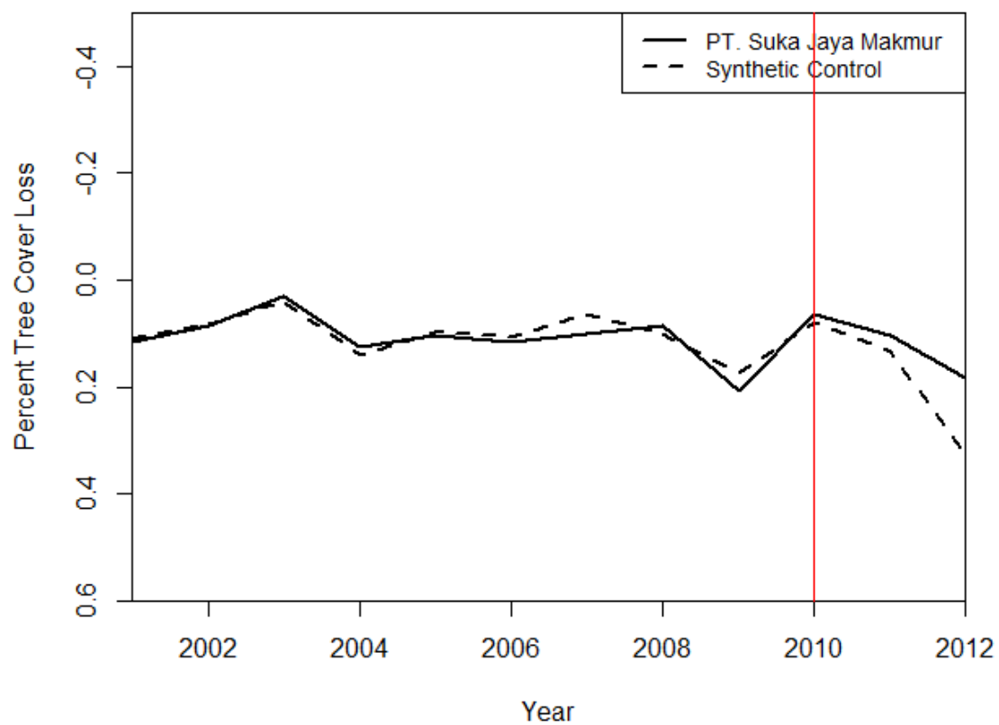
Figure 4. Comparison of tree cover loss in Suka Jaya Makmur and its synthetic control, 2001–2012. Tree cover loss increases down the y -axis. Red line indicates the year of certification.
