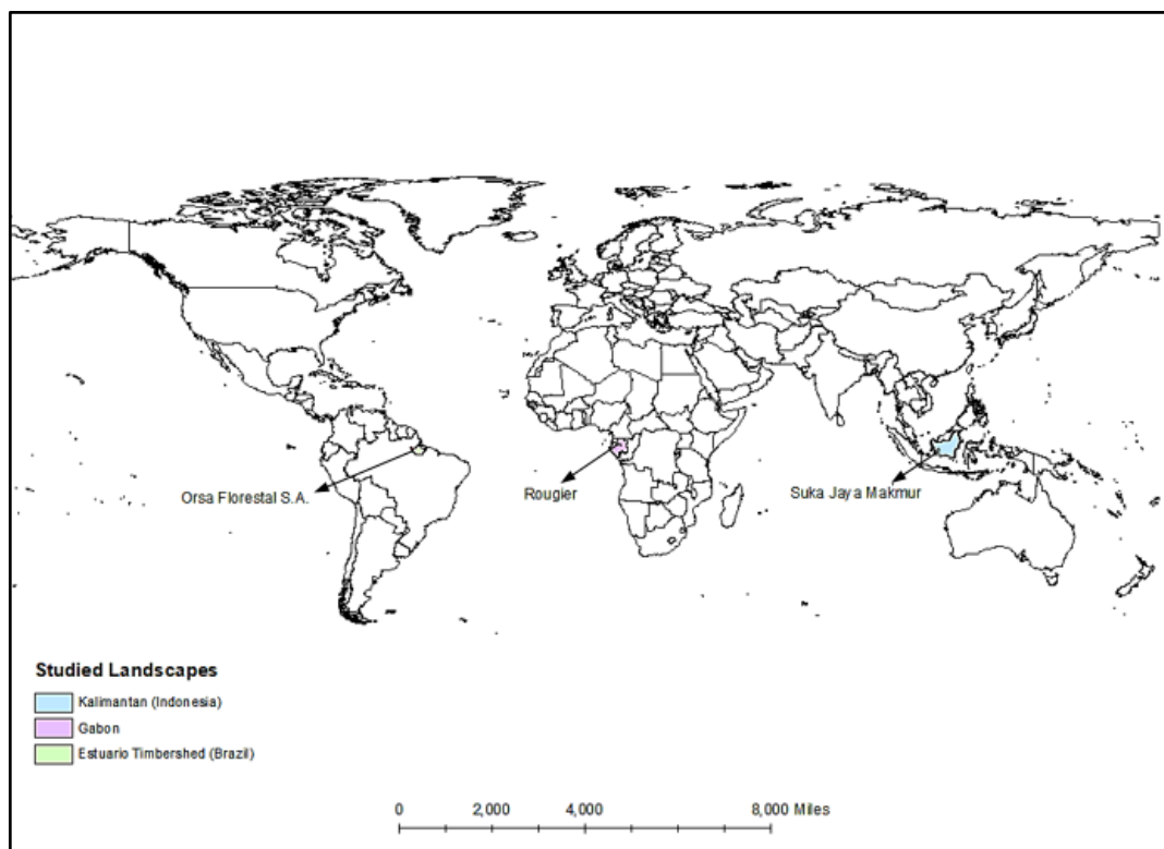
Figure 1. Locations of Orsa Florestal S.A., Rougier, and Suka Jaya Makmur in studied landscapes.
