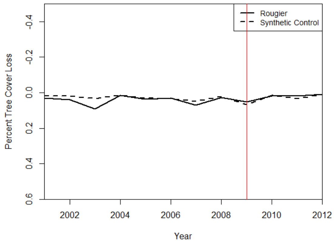
Figure 3. Comparison of tree cover loss in Rougier and its synthetic control, 2001–2012. Tree cover loss increases down the y -axis. Red line indicates the year of certification.
