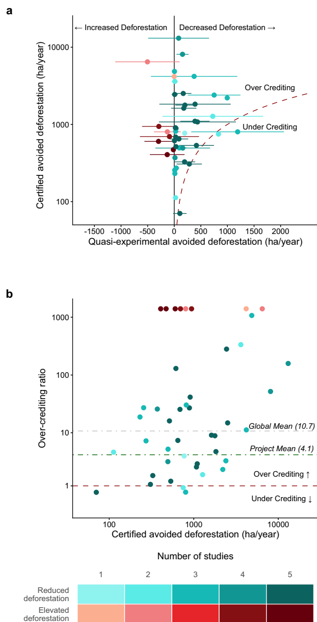
Fig. 2 | Comparison of quasi-experimental and certified estimates of project performance. a Quasi-experimental evaluations show consistent evidence that REDD+ projects slowed deforestation, but certified estimates were higher, indicating widespread over-crediting. Points represent mean estimates from the six quasi-experimental studies, with error bars showing 95% confidence intervals. b The over-crediting ratio (the certified estimate divided by the mean quasi-experimental estimate) plotted against certified avoided deforestation estimates. The dashed grey line indicates the global mean over-crediting ratio and the dashed red lines mark parity between certified and quasi-experimental estimates. Points above and below the red line represent over- and under-crediting respectively. Darker colours denote projects evaluated by a greater number of quasi-experimental approaches (up to five as there was no overlap in the projects assessed by the two West et al. studies). The over-crediting ratio is undefined for the points that experienced more deforestation than predicted by their quasi-experimental controls (shown in red). Both panels use log-scaled y-axes.
