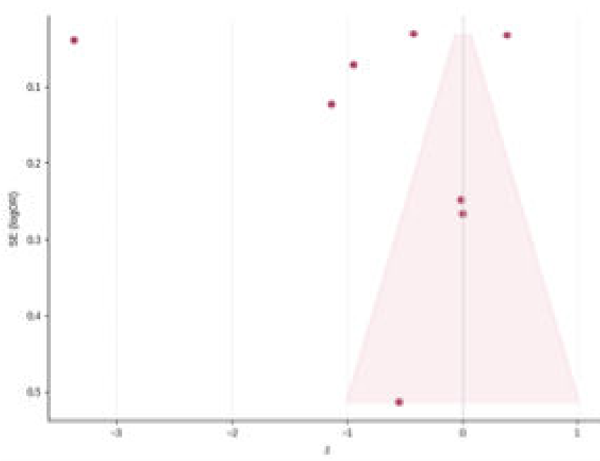
Figure 10. Funnel plot to assess publication bias for annual deforestation rate studies
